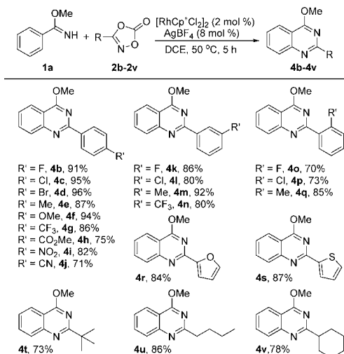
Scheme 3. Reaction Scope for Dioxazolones a,b
